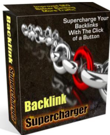
Backlink Supercharger
